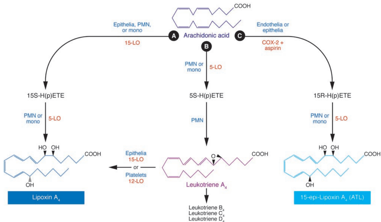
Figure 1 Lipoxin biosynthesis. There are at least 3 different biosynthetic pathways for lipoxin generation. All lead to the insertion of molecular oxygen at 2 sites in arachidonic acid by a variety of different enzymes that are generally segregated in different cell types and subject to regulation by cytokines and other inflammatory stimuli. In the first pathway (A), LXA 4 is generated through the action of 15-LO from airway epithelia or myeloid cells (neutrophils, monocyte/macrophages), which is followed by the action of 5-LO in myeloid cells. In the second pathway (B), LXA 4 is generated from leukotriene A 4 (LTA 4 ) (itself a product of 5-LO activity, and a leukotriene precursor) through the action of 15-LO or platelet-derived 12-LO. In the third pathway (C), arachidonic acid is converted to aspirin-triggered lipoxins (ATLs) such as 15-epi-LXA 4 , via the action of epithelial or endothelial COX-2 in the presence of aspirin, which is followed by the action of 5-LO. The ATLs have similar activities but greater functional potency due to their relative resistance to metabolic inactivation. These pathways likely operate both independently and in a coregulated fashion in different tissues and biological situations. H(p)ETE, hydroperoxyeicosatetraenoic acid; mono, monocyte/macrophage; PMN, polymorphonuclear neutrophil.
