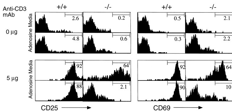
Figure 6 Effect of adenosine on TCR-triggered upregulation of CD25 and CD69 activation markers in vitro. Ex vivo spleen cells from ADA -/- and ADA +/+ littermates were incubated in 96-well plates with immobilized anti-CD3 mAb (5 μg/ml mAb) or with serum-free, ADA-free media alone (0 μg/ml mAb) in the presence or absence of adenosine (100 μM); 16 hours later, TCR-triggered upregulation of the T cell activation markers CD69 and CD25 was evaluated by flow cytometry.
